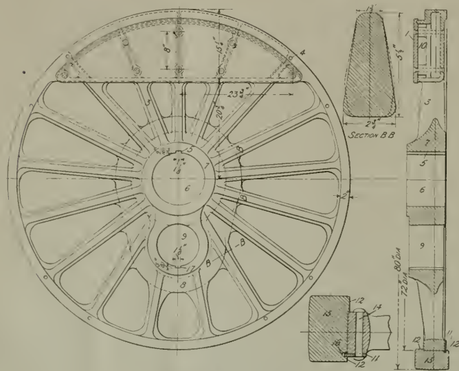
MAIN DRIVING WHEEL.
